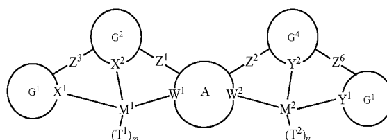
Formula (IV)
